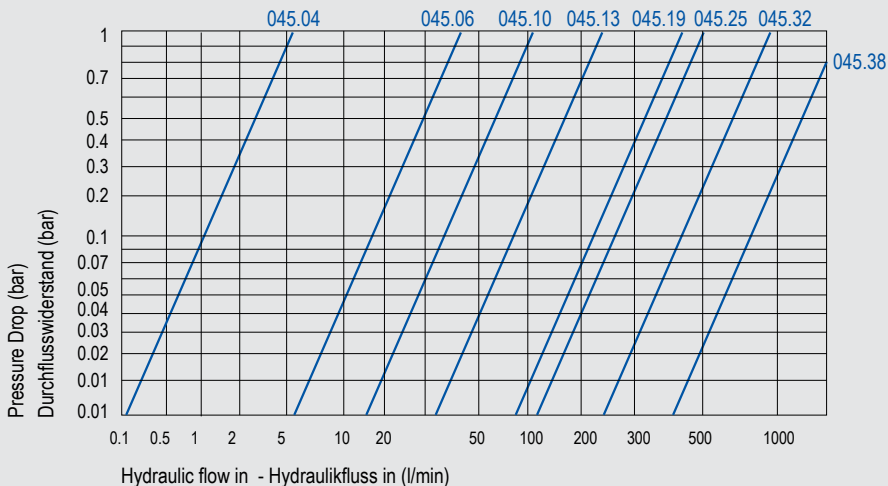
Flow Rate vs Pressure Drop Graph
